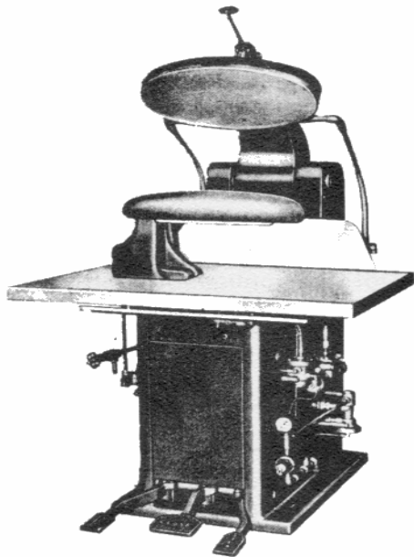
MODEL AAM-1 - "ULTRAMATIC" AUTOMATIC AIR OPERATED MUSHROOM TOPPER FOR LADIES' SLACKS
