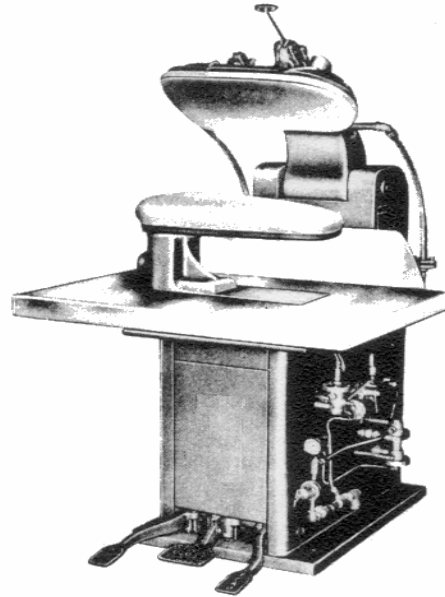
MODEL AAT-11 - "ULTRAMATIC" AUTOMATIC TROUSSE TOPPER
