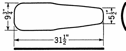
MODEL U-4 This model is used for the same operation as the U-3. Head and buck, which are oval, are desired by some manufacturers because of the contour of the buck.
