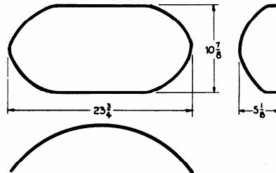
MODEL H-2 Especially designed to form the modern hip formation which is so widely used by ladies' suit manufacturers. It is used to offpress the hip section after the hip canvas is basted to the coat, or for shaping the canvas separately.
