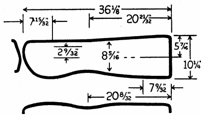
MODEL U-6 (Right and Left): For pressing back seams and shoulder blades on young men's coats. It will press the shape needed for the shoulder blade as well as the curvature between the shoulder and waist.
