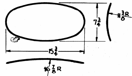
MODEL M-7 Shorter and narrower than older mushroom designs, for pressing ladies' form fitting woolen dresses, blouses and tailored jackets with ease and speed. Used for shaping upper back portion and the hip, as well as finishing the bottom of ladies' jackets.
