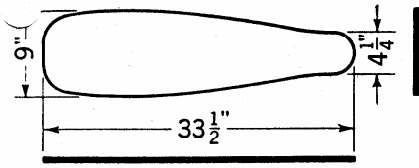
MODEL U-3 Used in conjunction with front offpressing. Will finish sides and backs of men's sack coats without destroying the chest expression as often happens with wider machines. Has a flat pressing surface.
