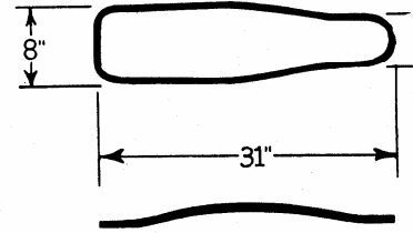
MODEL U-5 The head and buck of this model are designed as a back pressing machine. They have a special contour and is especially desirable for ladies' shape coats. Also used for children's jackets.
