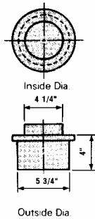
M-2010 (4 1/4" - 5 3/4")
