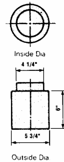
M-2030 (4 1/4" - 5 3/4")
