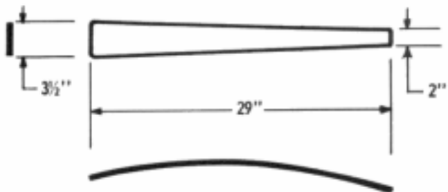
Model S-21 is designed to press the elbow seams on mens sack coats, topcoats and overcoats before or after underseam is joined.
