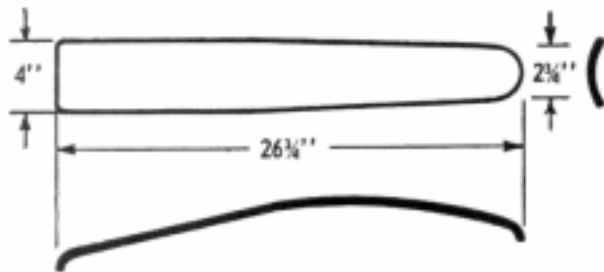
Model S-5 is designed for pressing the elbow seams on top coats and overcoats before or after under seam is joined.
