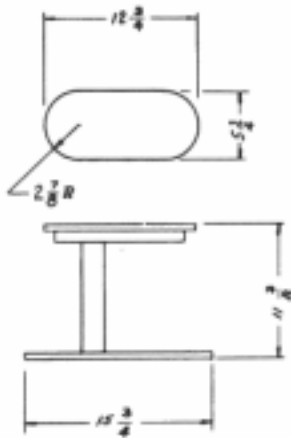
MODEL J-58-H MODEL S-58-N Flat Sleeve Blocker to block the upper portion of sleeves of sackcoats, topcoats and overcoats. Suitable for manufacturing and alteration plants.
