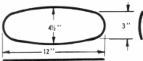
MODEL J-18-H MODEL S-18-N Utility Blocker designed for creasing armholes and pressing the upper portions of sleeves on sackcoats, topcoats and overcoats. Suitable for alteration rooms and manufacturing plants.
