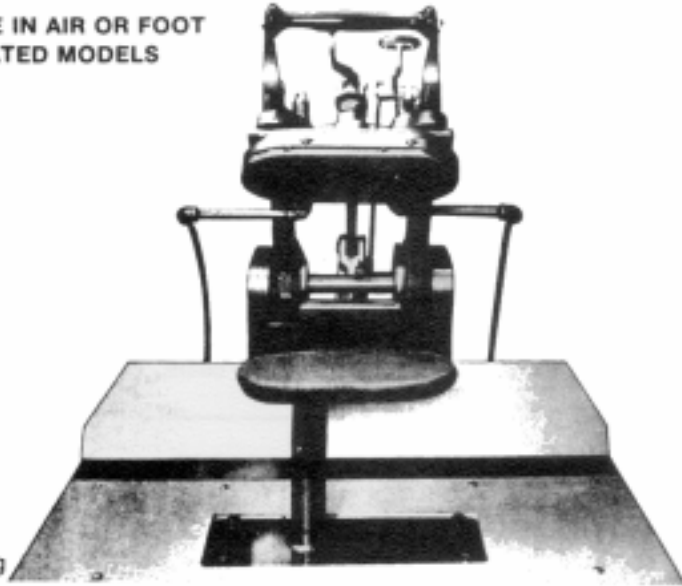
MODEL J-58-H MODEL S-58-N Flat Sleeve Blocker to block the upper portion of sleeves of sackcoats, topcoats and overcoats. Suitable for manufacturing and alteration plants.
